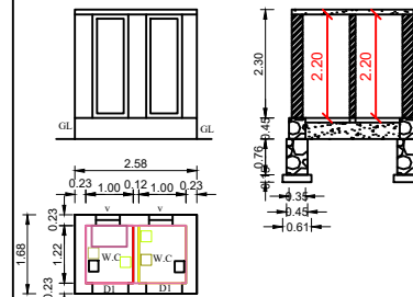
BATH ROOM PLAN
