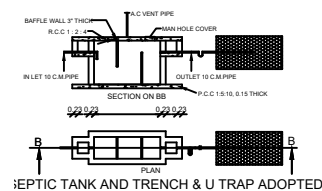
SEPTIC TANK AND TRENCH &amp; U TRAP ADOPTED
