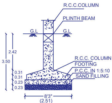
FOUNDATION DETAIL
