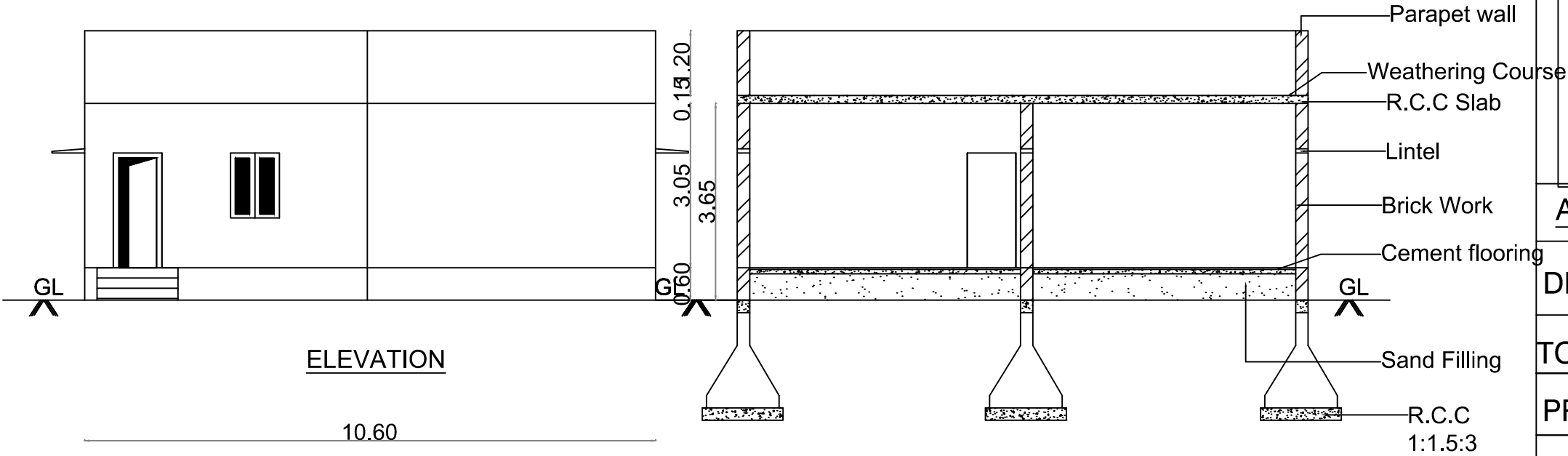
CROSS SECTION"AB"
