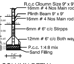
COLUMN DETIAL
