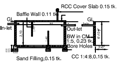
SEPTIC TANK & SOAK PIT
