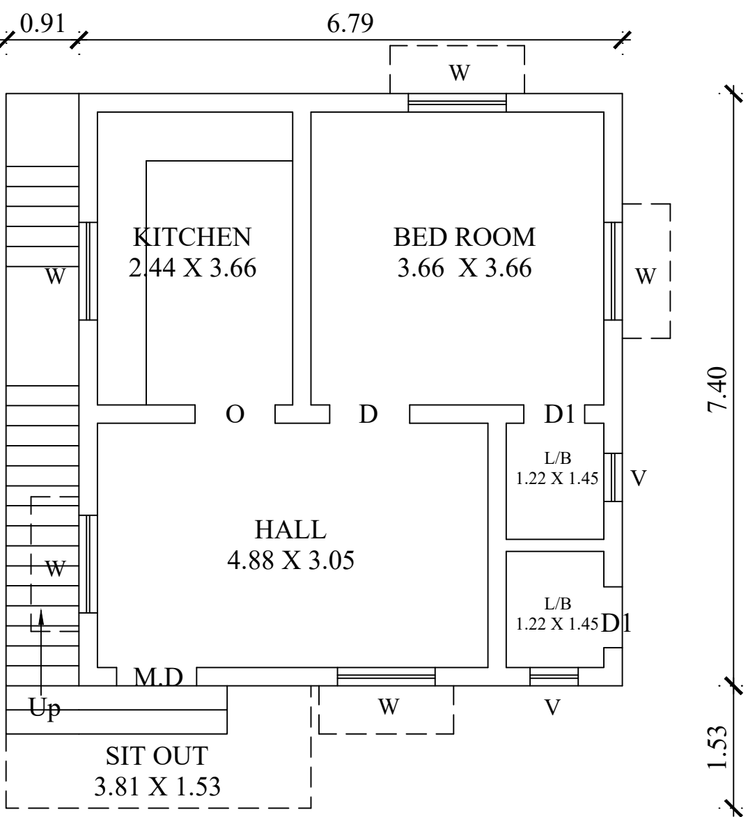
PROPOSED BUILDING PLAN - G.F
