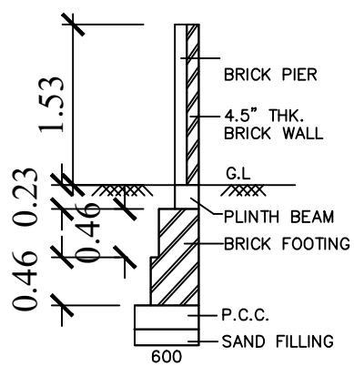
COMPOUND WALL DETAILS - N.T.S
