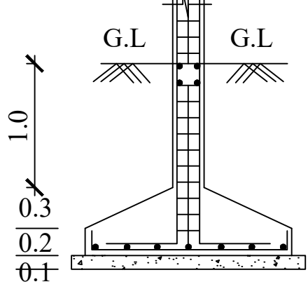
COLUMN FOOTING DETAILS - N.T.S
