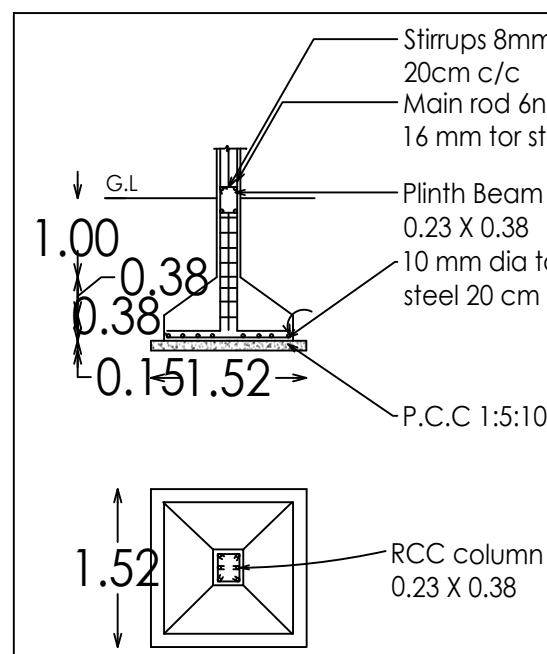
DETAILS OF COLUMN FOOTING
