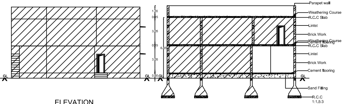
CROSS SECTION"AA"
