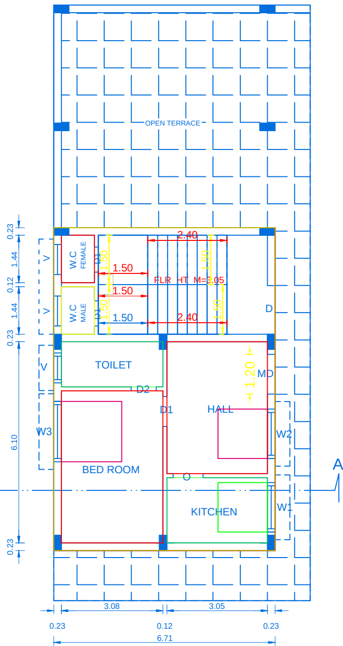
PROP.SECOND FLOOR PLAN
