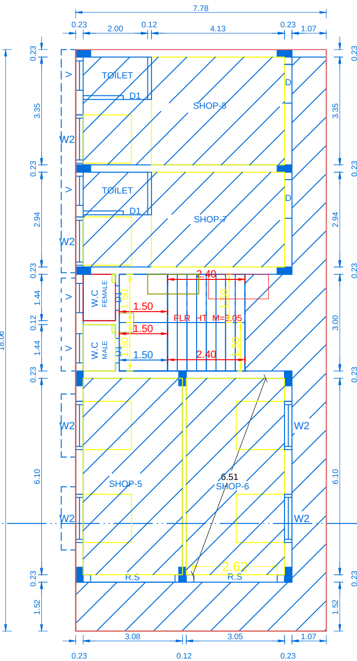
EXG.FIRST FLOOR PLAN
