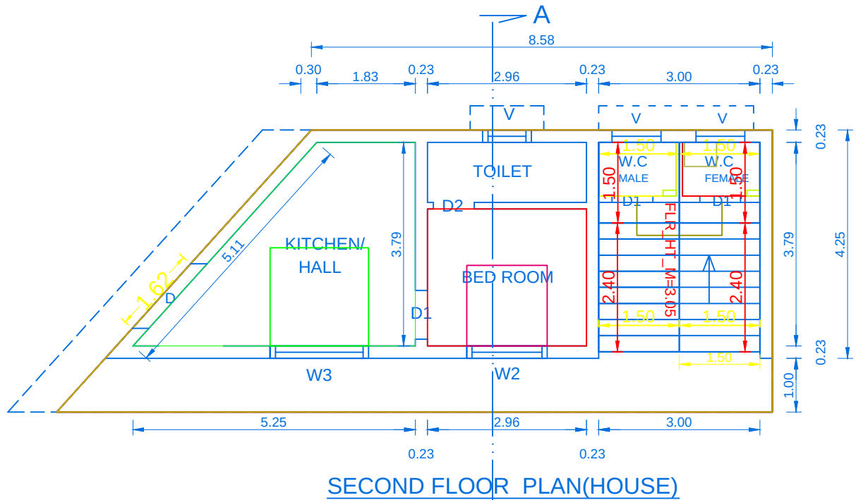
SECOND FLOOR PLAN(HOUSE)
