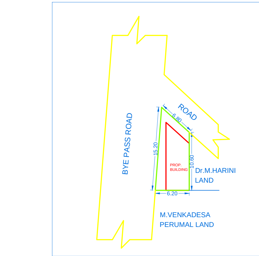
LOCATION PLAN Scale 1:400
