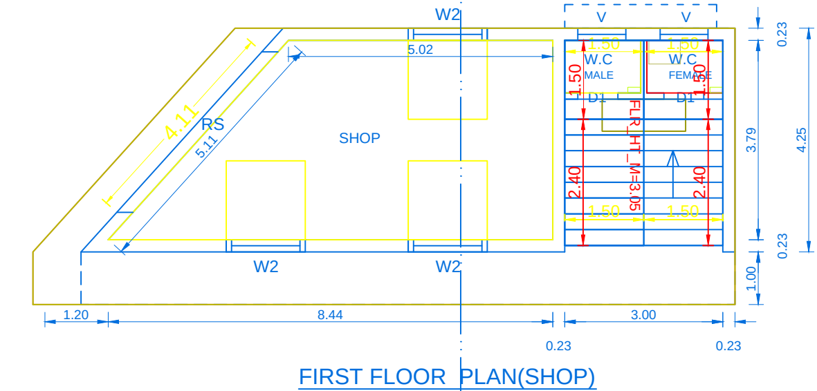
FIRST FLOOR PLAN(SHOP)
