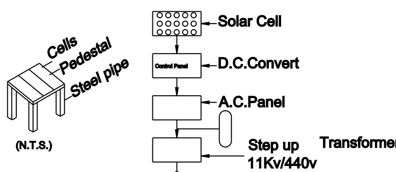
SOLAR SYSTEM FLOW DIAGRAM (7 - NOS PROVIDED)
