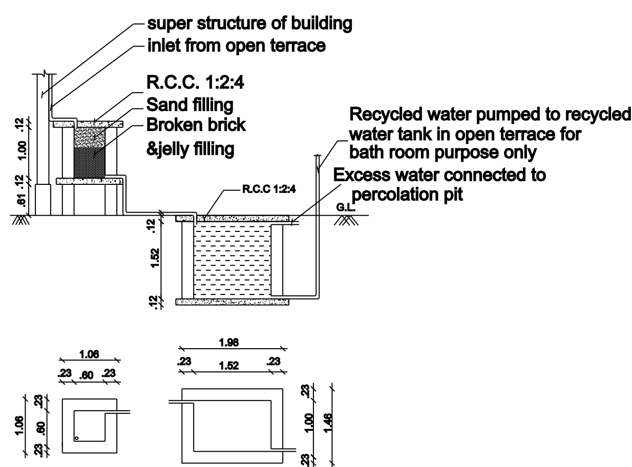
SUMP AND FILTER BED
