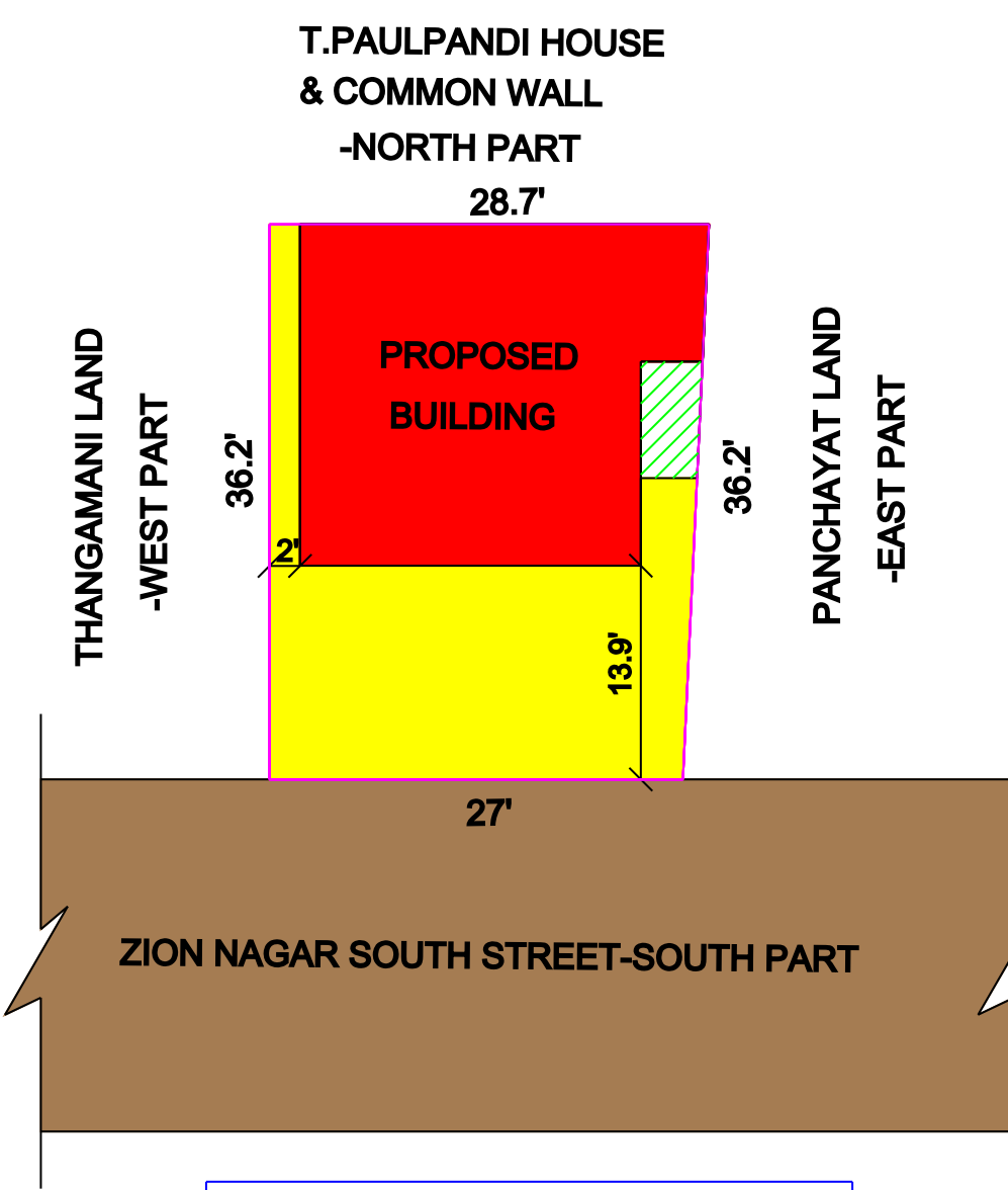
SITE CUM GROUND FLOOR PLAN SCALE 1: 200
