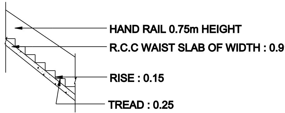
STAIRCASE DETAIL
