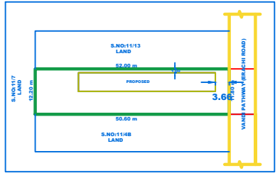
LOCATION PLAN
