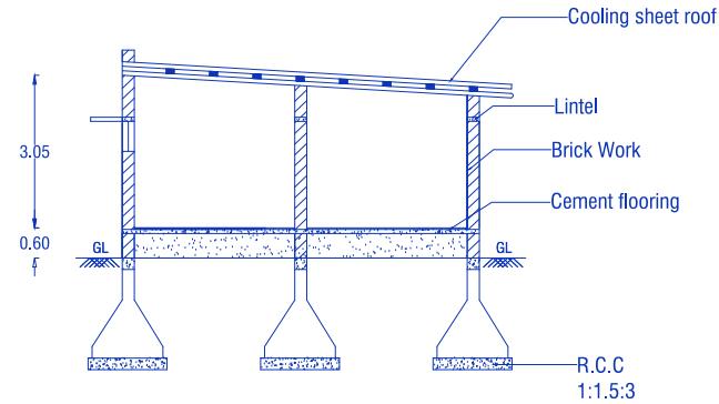
CROSS SECTION ON 'AB'
