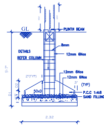
FOUNDATION DETAILS SCALE : 1:50.
