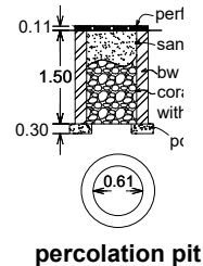
percolation pit
