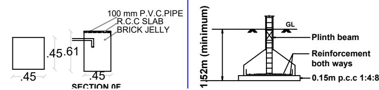
.DET.COLUMN FOOTING
