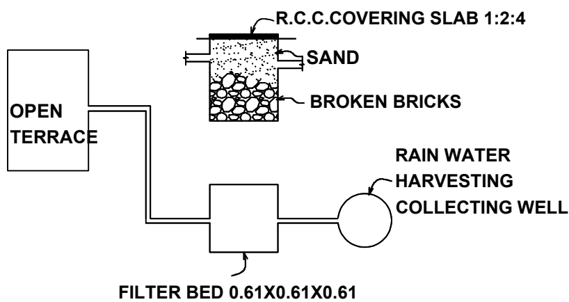
DETAILS OF RAIN WATER HARVESTING SYSTEM
