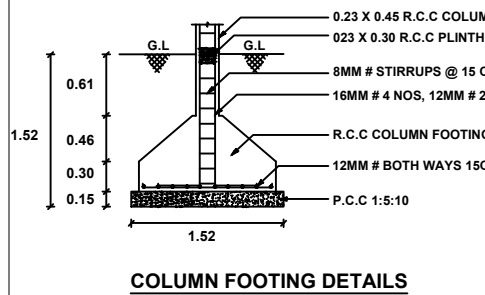
COLUMN FOOTING DETAILS
