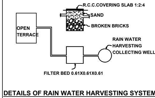
DETAILS OF RAIN WATER HARVESTING SYSTEM
