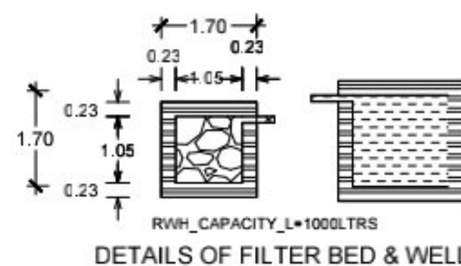
DETAILS OF FILTER BED & WELL
