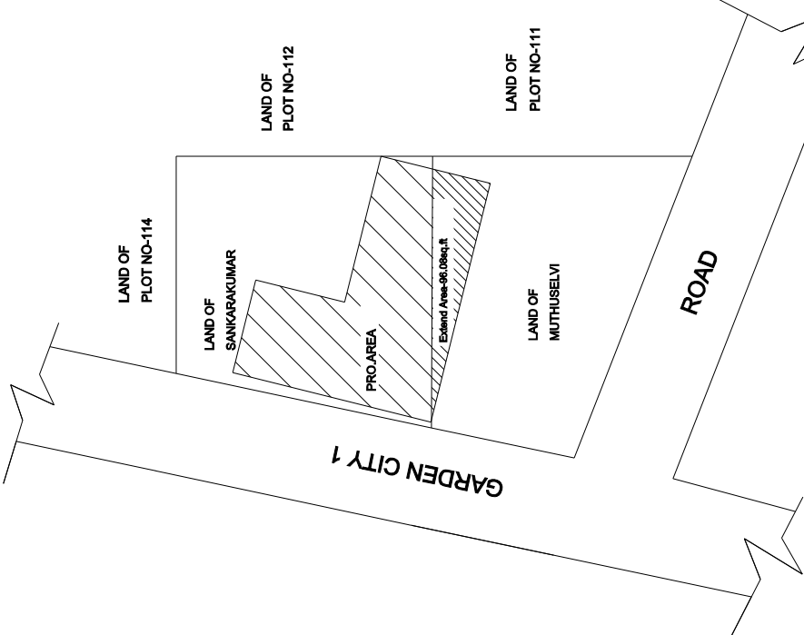
SITE PLAN
