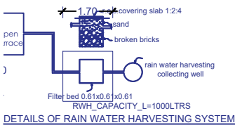
DETAILS OF RAIN WATER HARVESTING SYSTEM
