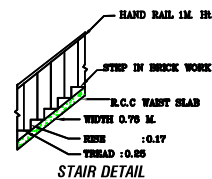
STAIR DETAIL
