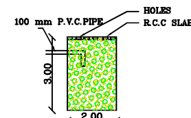
SECTION OF RAIN WATER COLLECTING TANK
