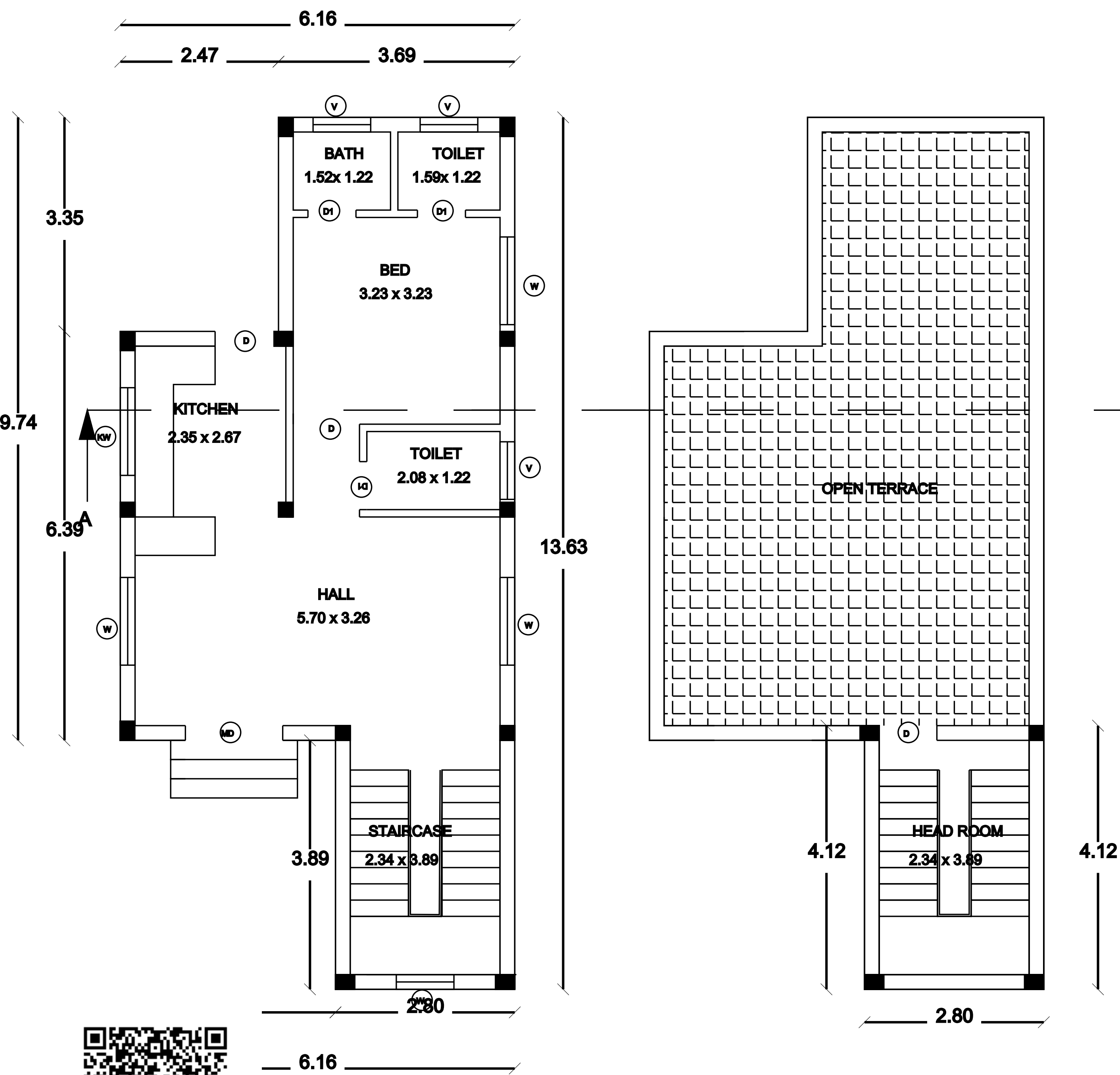
FLOOR PLAN
