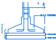
TYPICAL SECTION OF R.C.C COLUMN FOUNDATION
