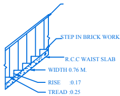
STAIR DETAIL
