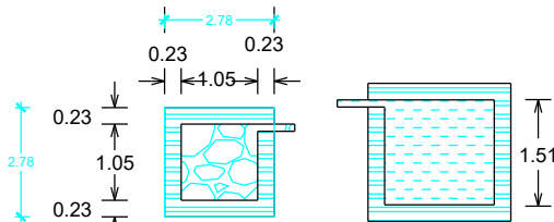
DETAILS OF FILTER BED & WELL
