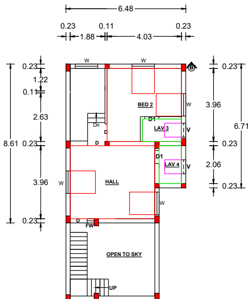
FIRST FLOOR PLAN (SOUTH FACING )
