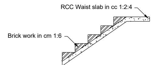
STAIRCASE DETAILS
