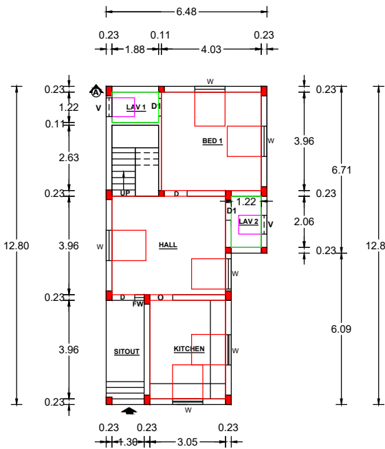
GROUND FLOOR PLAN (SOUTH FACING )
