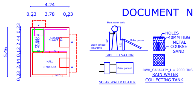
PROPOSED FIRST FLOOR PLAN(HOUSE I)
