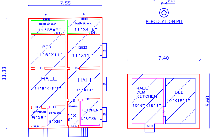
HOUSE-I HOUSE-II HOUSE-III EXG- GROUND FLOOR
