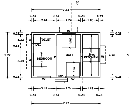
GROUND FLOOR PLAN -(HOUSE-II)
