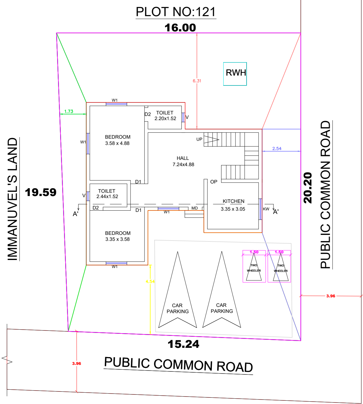
SITE PLAN
