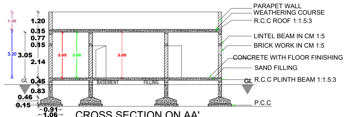
CROSS SECTION ON AA'
