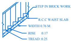
STAIR DETAIL
