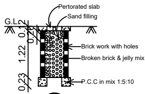
section of compound wall details
