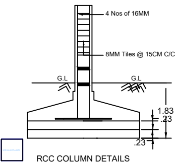
RCC COLUMN DETAILS
