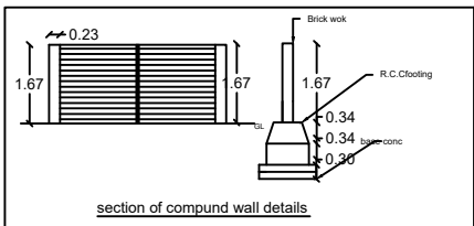
section of compound wall details
