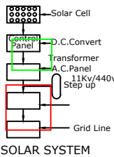
SOLAR SYSTEM
