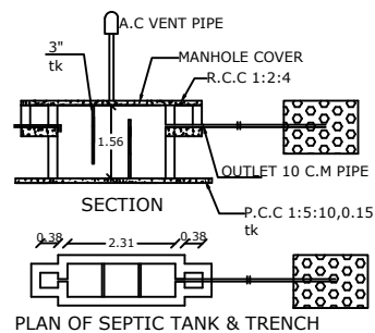
PLAN OF SEPTIC TANK & TRENCH
