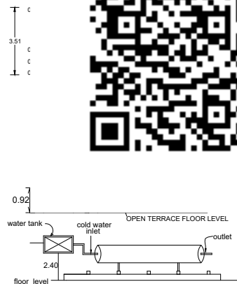
Details of solar water heating system
