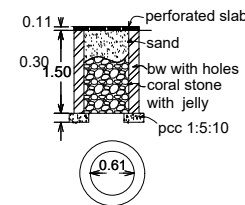
percolation pit
