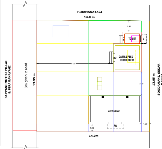
SITE PLAN
