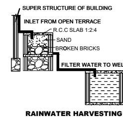
RAINWATER HARVESTING
