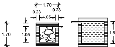
DETAILS OF FILTER BED & WELL
