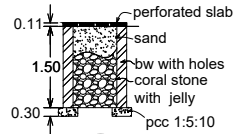
percolation pit
