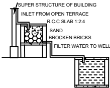
RAINWATER HARVESTING
