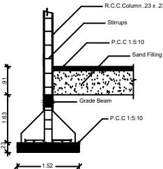
COLUMN DETAIL
