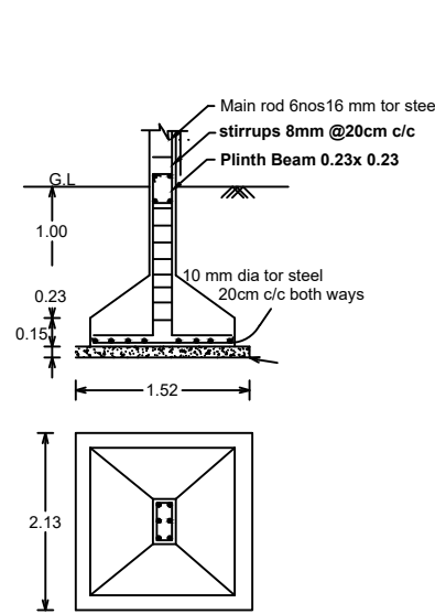
Details of column footing
