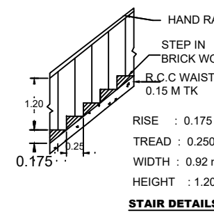
STAIR DETAILS
