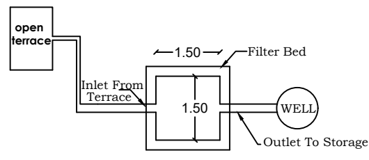
Plan Of Filter Bed & Well
