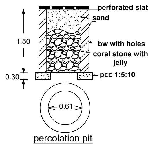
perforated slab
