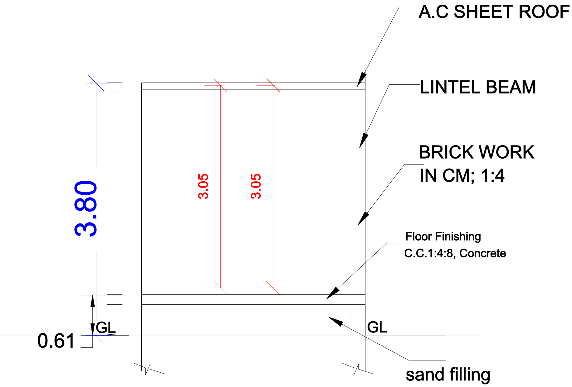
SECTION NN
