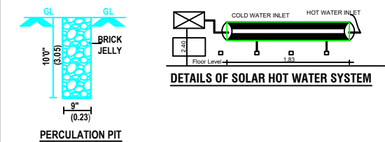
PERCOLATION PIT
