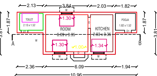
PRO GROUND FLOOR
