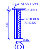
PERCOLATION PIT DETAILS OF JOINERIES:-
