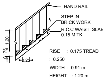
STAIR DETAILS
