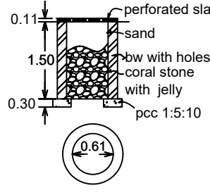
PERCOLATION PIT
