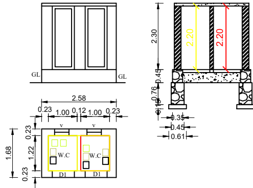
BATH ROOM PLAN
