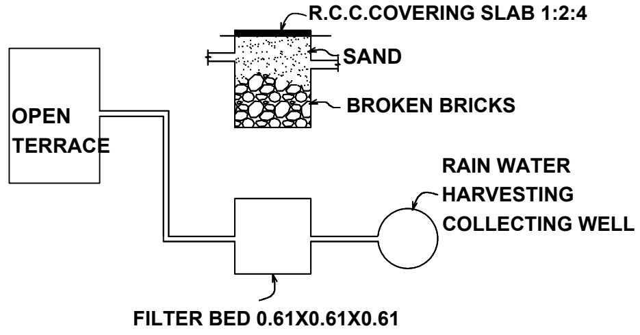
DETAILS OF RAIN WATER HARVESTING SYSTEM
