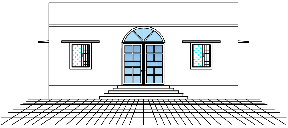
FRONT ELEVATION.
