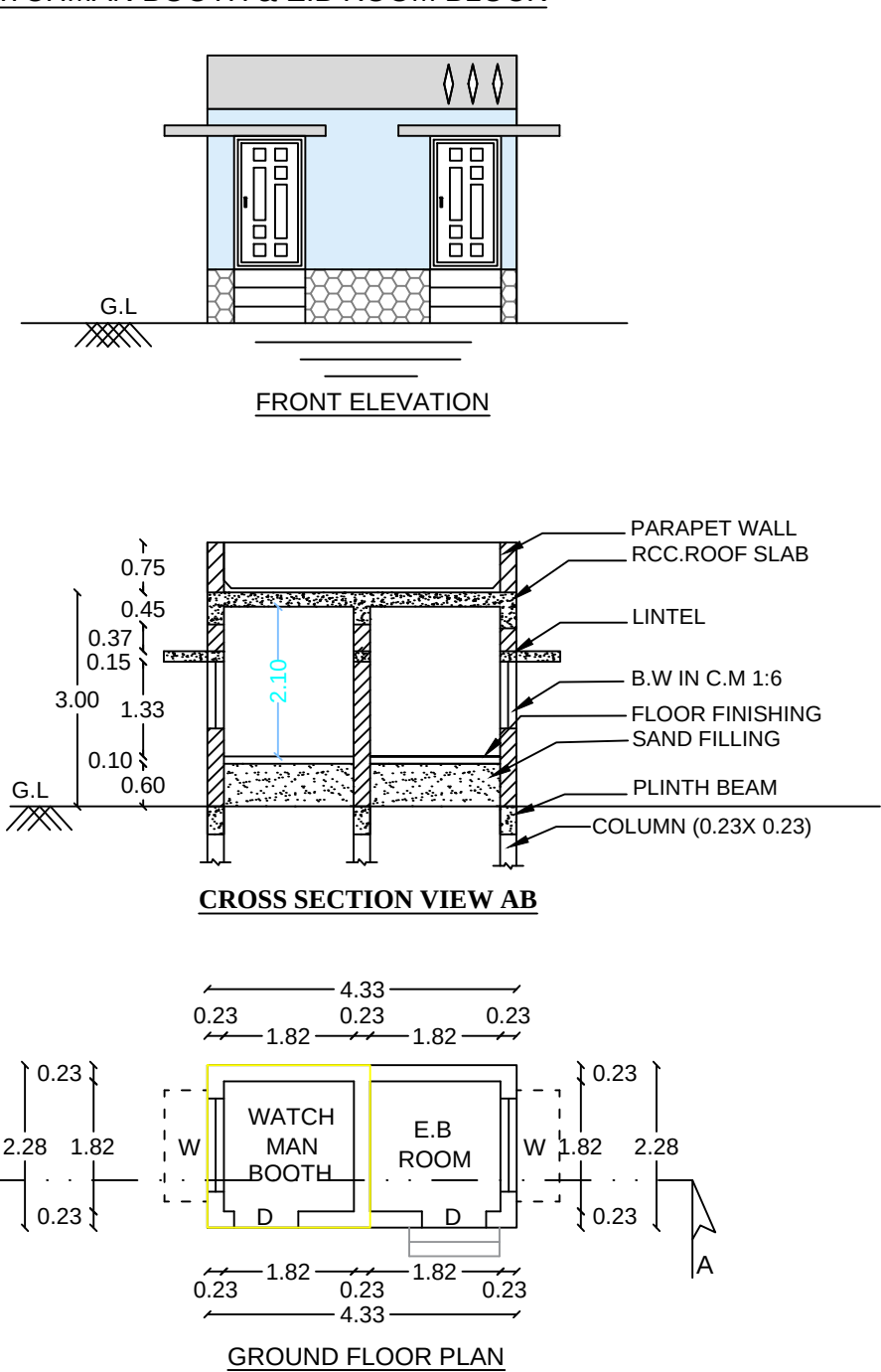
WATCHMAN BOOTH & E.B ROOM BLOCK
