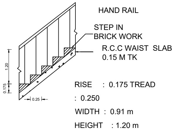
STAIR DETAILS
