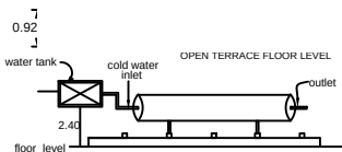
Details of solar water heating system
