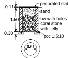
percolation pit
