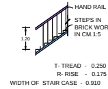
DETAILS OF STAIRCASE
