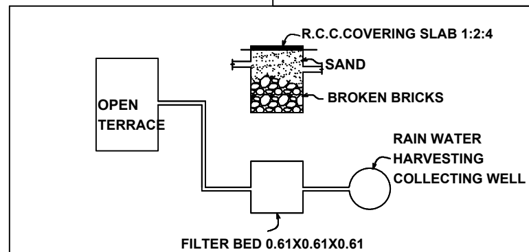
DETAILS OF RAIN WATER HARVESTING SYSTEM
