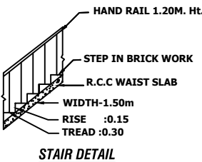
STAIR DETAIL
