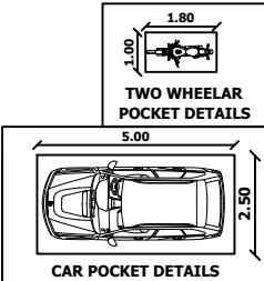
CAR POCKET DETAILS
