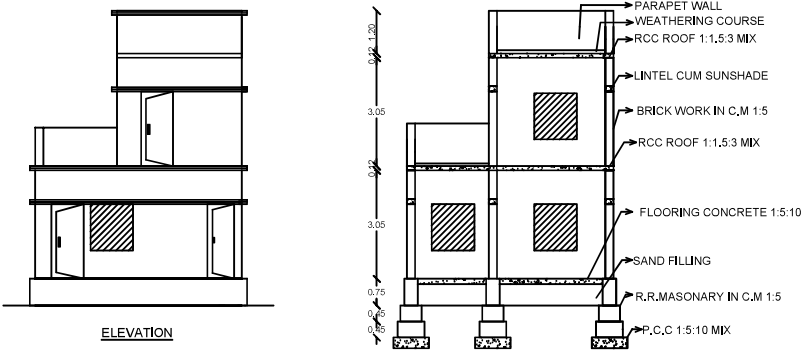
SECTION ON ABCD
