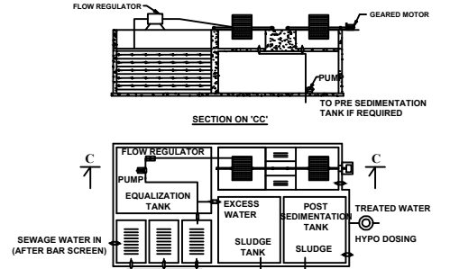
DETAILS OF SEWAGE TREATMENT PLANT
