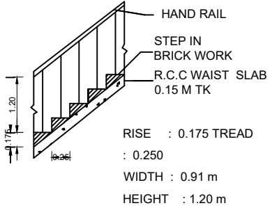
STAIR DETAILS
