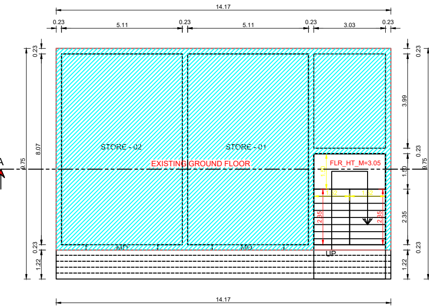
EXS.GROUND FLOOR PLAN
