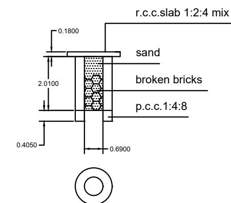
PERCOLATION PIT
