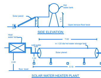
SOLAR WATER HEATER PLANT
