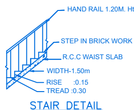
STAIR DETAIL
