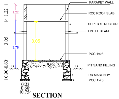
SECTION
