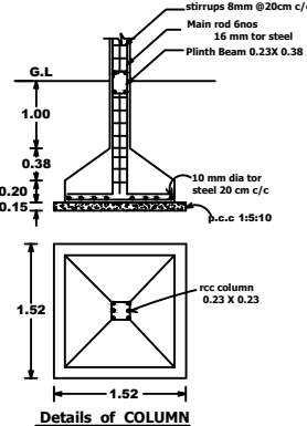
Details of COLUMN
