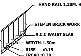
STAIR DETAIL
