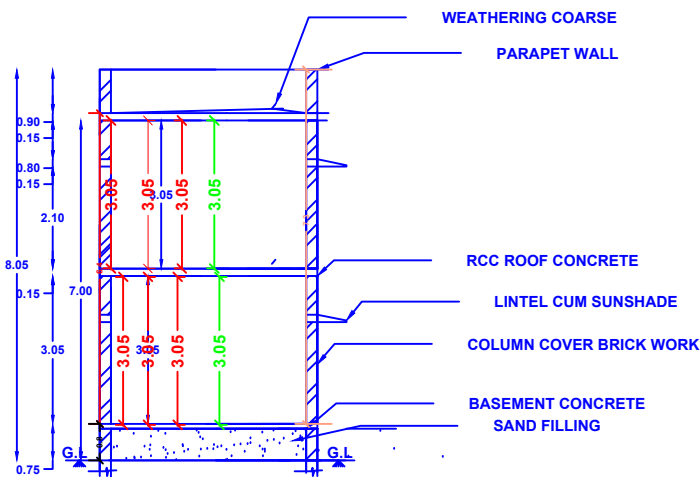
SECTION AB
