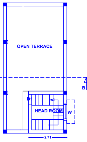
TERRACE PLAN
