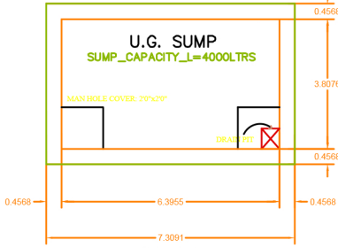
SUMP DETAIL
