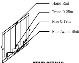
STAIR DETAILS
