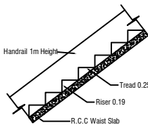
STAIR DETAILS
