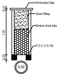
RAIN WATER COLLECTION WELL
