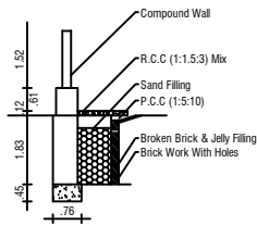
RAIN WATER HARVEST DETAILS
