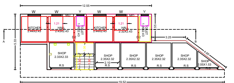
EXI-CUM-PRO.GROUND FLOOR PLAN
