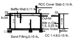
SEPTIC TANK & SOAK PIT
