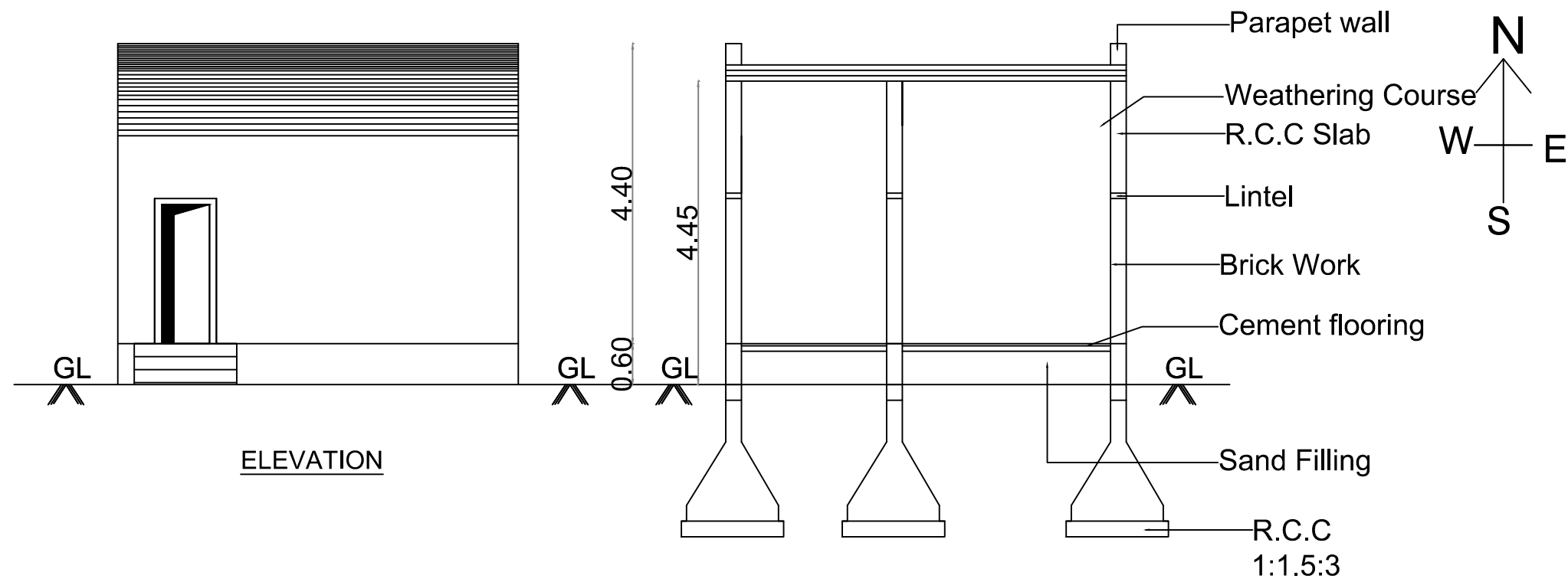
CROSS SECTION"AA"
